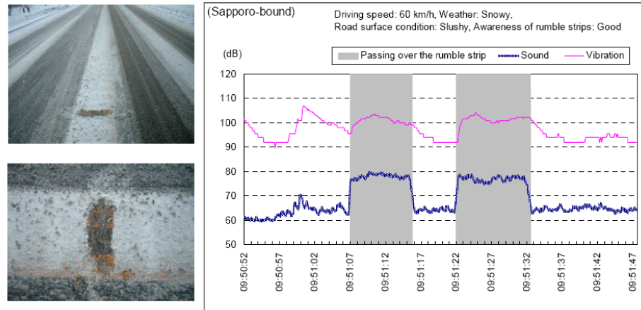
Figure A-7. Sound and Vibration Measured on National Route 274 During Winter Conditions (42)
